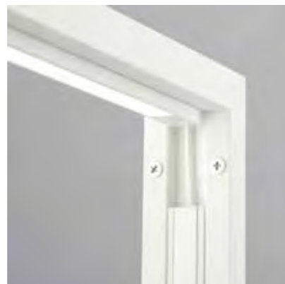
When using LED lighting strip in the frame, the cables are led through the frame interior into the cable box and then to a socket.
